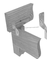
Typical RT7A-TZ installation
